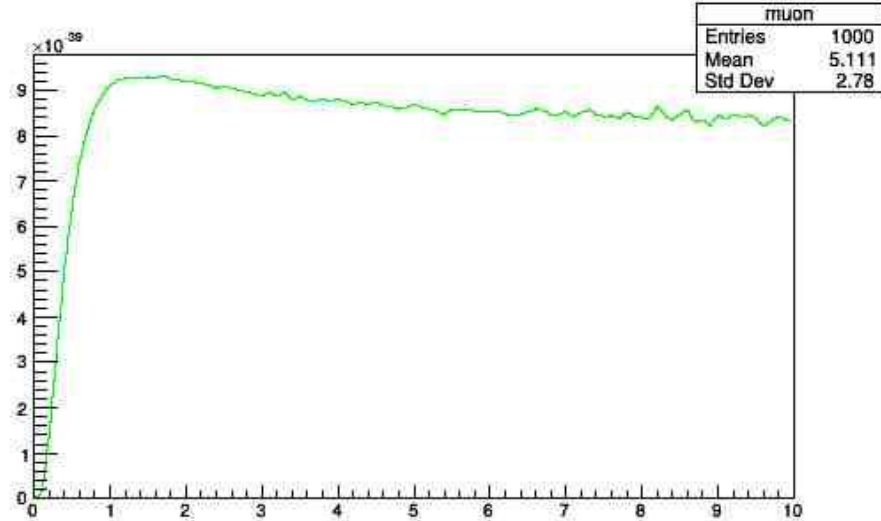
muon-Carbon
