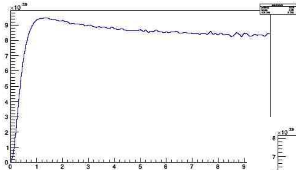
electron-Argon
