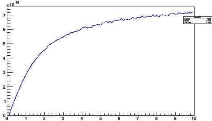
antimuon-Oxygen
