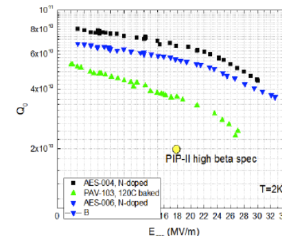
PIP-II cavity performance after N doping
